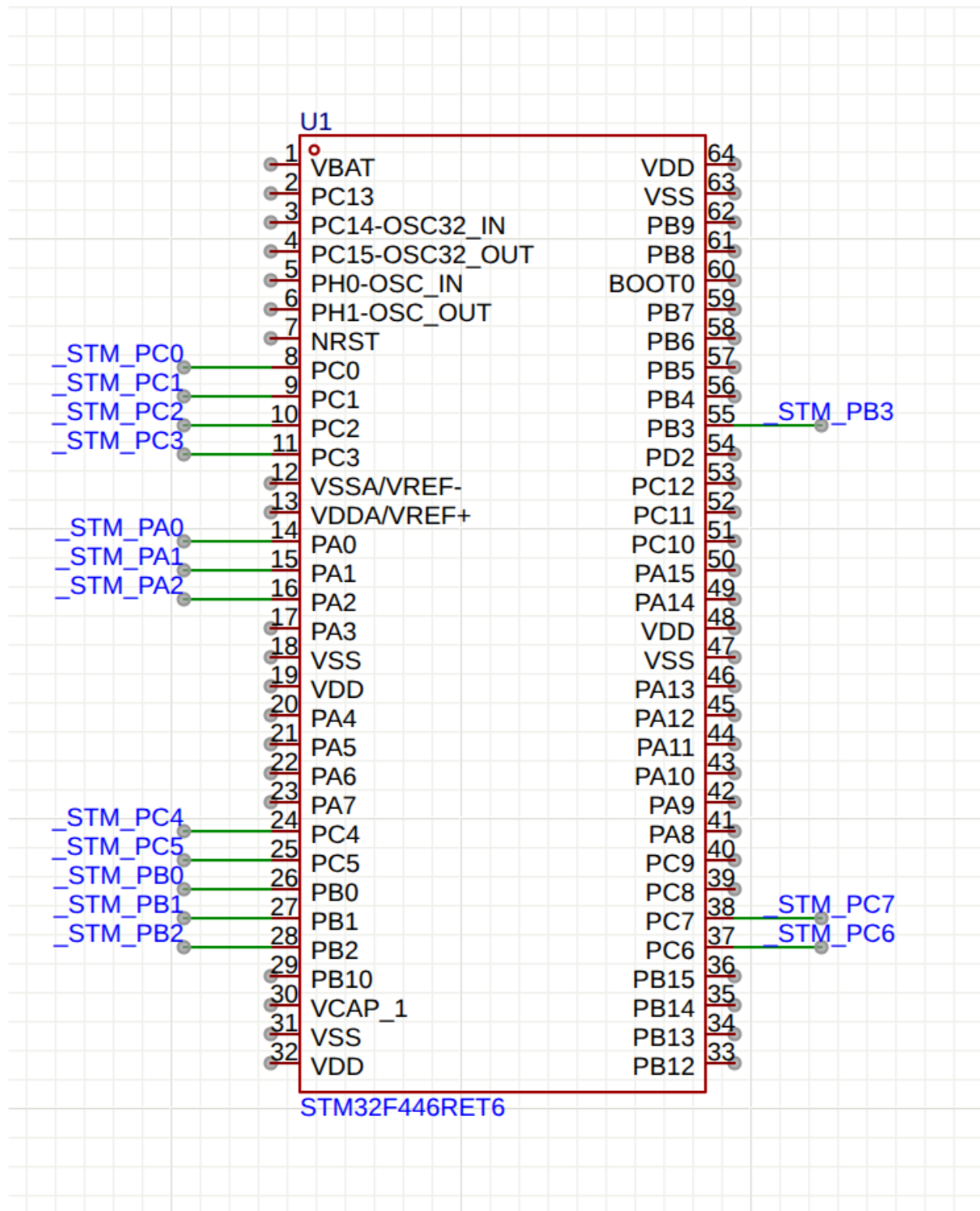
Figure 3.4 STM32 Connection
