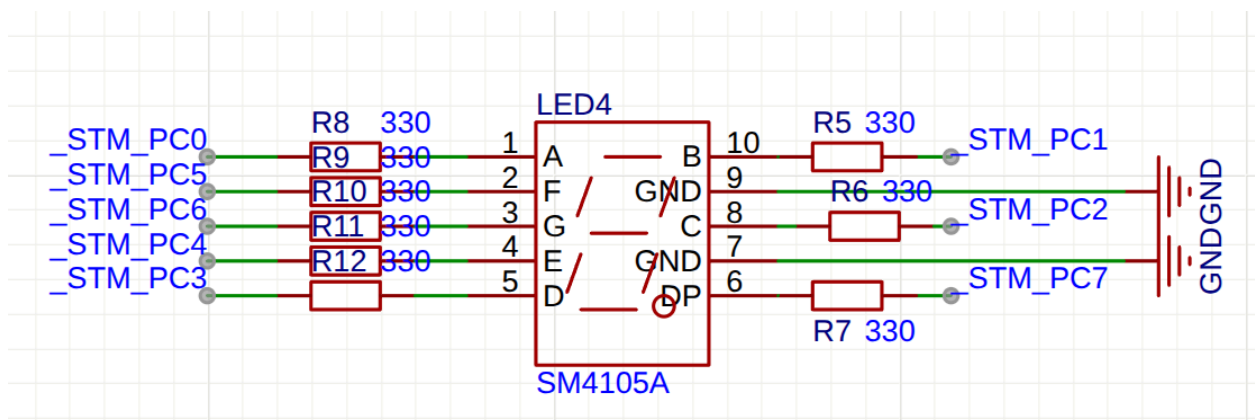
Figure 3.3 7 Segment Connection
