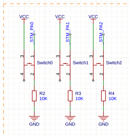
Figure 3.1 Active High Push Button
