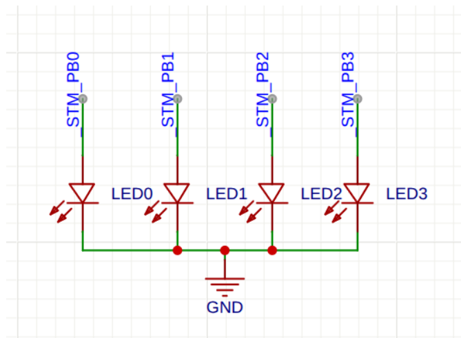
Figure 3.2 Common Cathode LEDs
